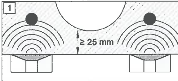
1 Locate rebars by means of suitable detector
