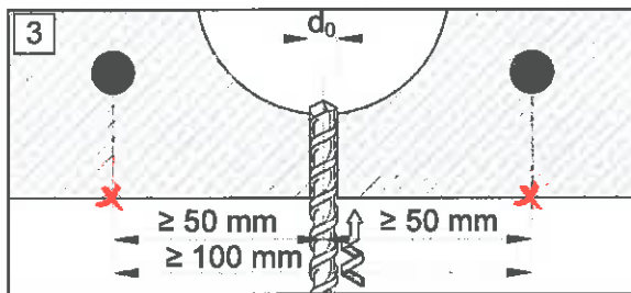
3 Make a cylindrical hole
